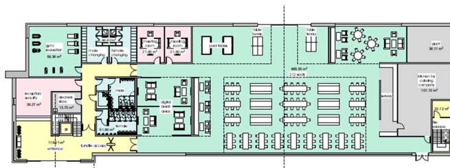
proposed ground floor plan 1:200
